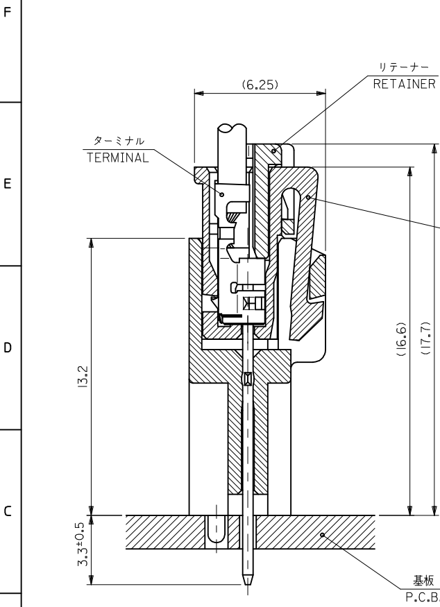
嵌合断面図 (参考) LAYOUT OF EACH CKTS.
