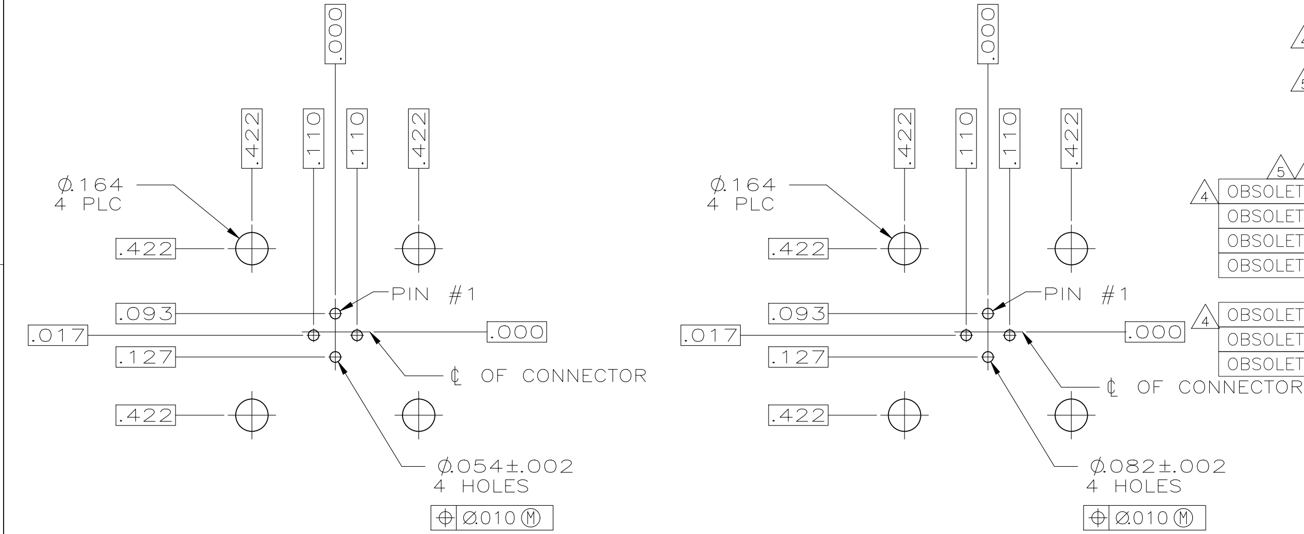
RECOMMENDED P.C. BOARD LAYOUT
