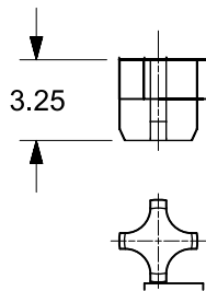
PRESS-FIT PEG
