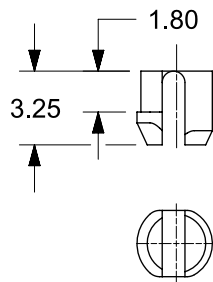
SNAP-FIT PEG
