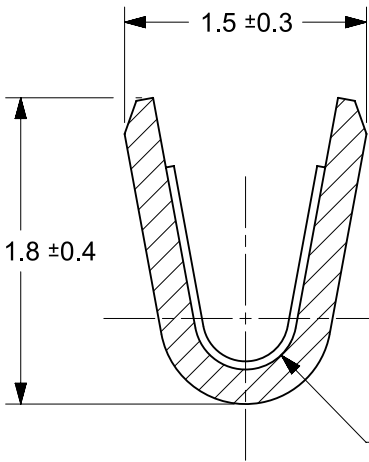
SECTION Y-Y
