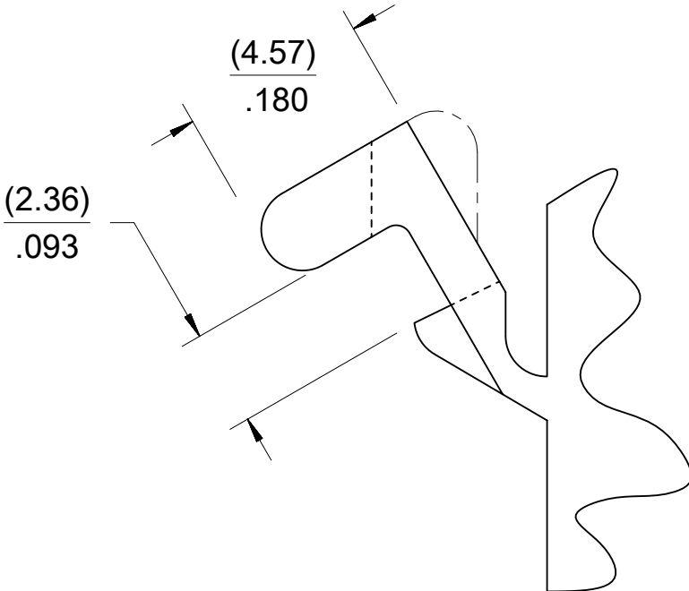
DETAIL 1 .093/(2.36) PREBENT MOUNTING EAR
