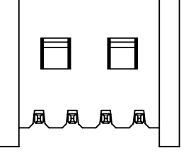
1 4~15極形状 (2ロック) FIGURE OF 4-15 CIRCUIT (2 LOCKS)
