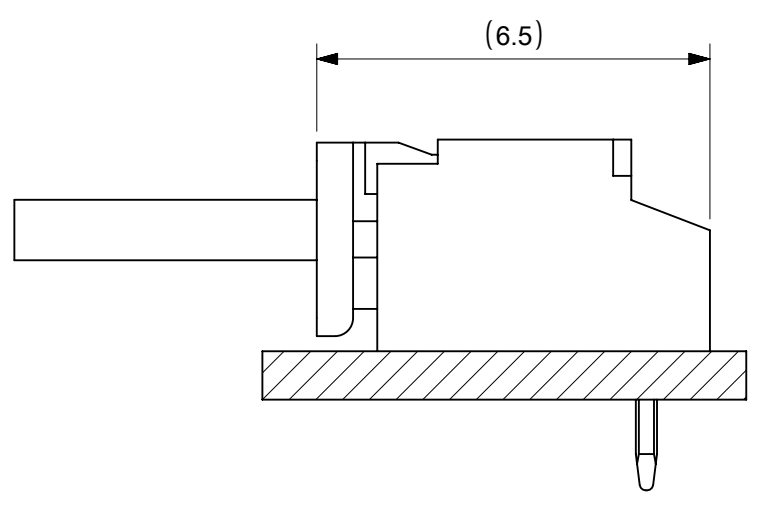
1 2, 3極形状 (1ロック) FIGURE OF 2, 3 CIRCUIT (1 LOCK)
