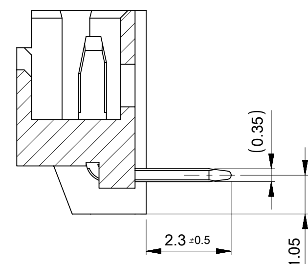
SECTION X-X
