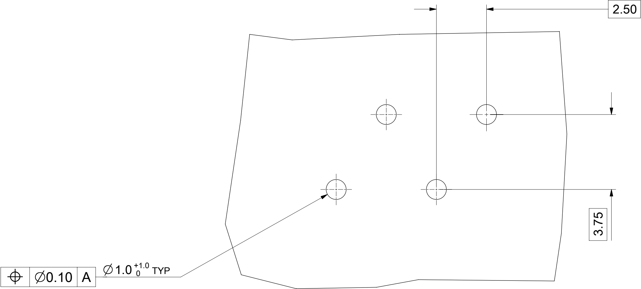
RECOMMENDED PCB LAYOUT FOR P/N: 93070-0521
