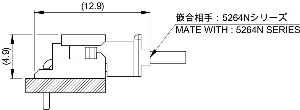
2-8極 2-8 CIRCUIT
