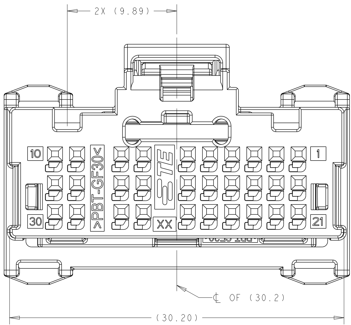
KEYING ARRANGEMENT VIEWS
