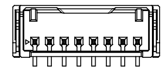
VIEW OF 7-8 CIRCUIT
